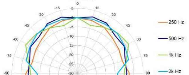
Directivity
